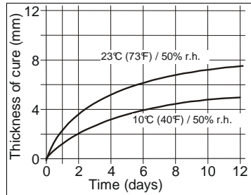
Diagram 1: Curing speed for Sikaflex ® -512 Caravan
